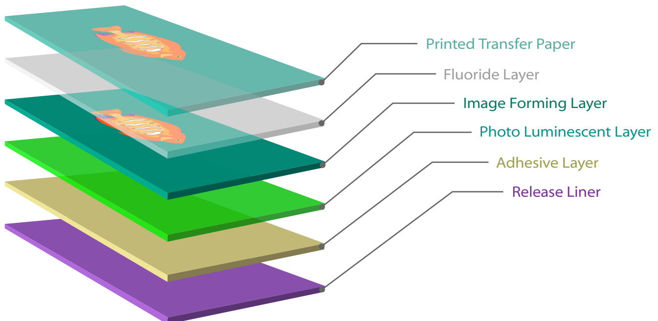
CROSS SECTION OF MEDIA
